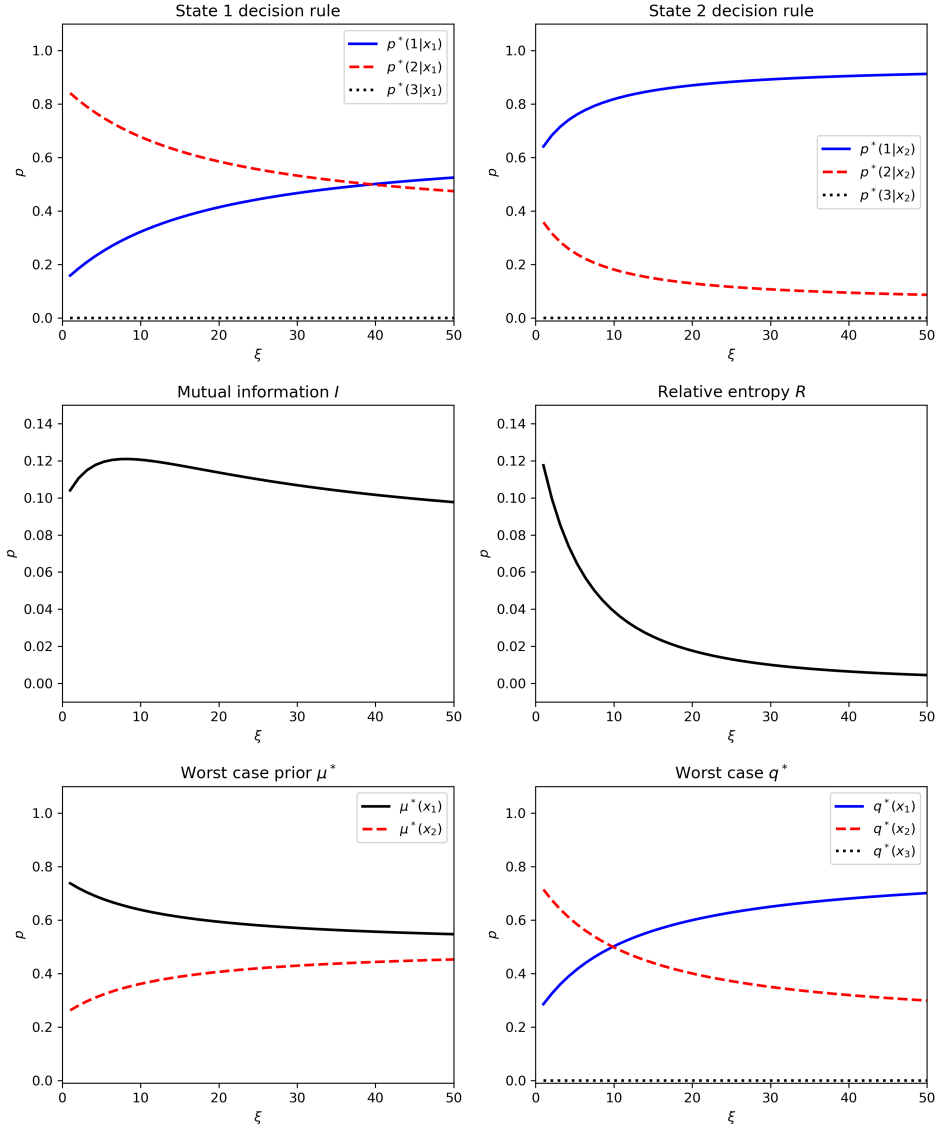
Figure 7: This figure explores the sensitivity to changes in \xi . The attention cost parameter, \lambda = 10 ; utility curvature parameter, \alpha = 0 , and r = 7.5 .
