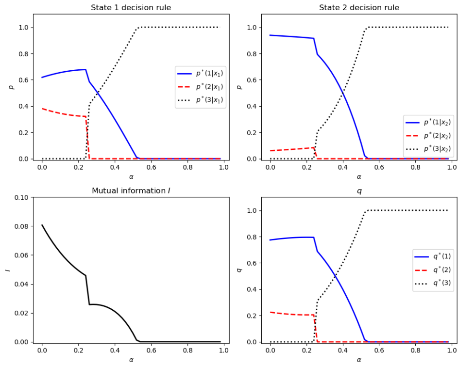
Figure 8: This figure explores the sensitivity to changes in \alpha . The attention cost parameter, \lambda = 10 ; robustness parameter, \xi = \infty , and r = 7.5 .
