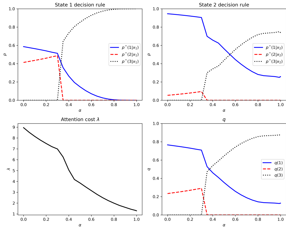
Figure 9: This figure explores the sensitivity to changes in \alpha . The mutual information is constrained by I \leq \kappa = 0.1 ; \xi = \infty and r = 7.5 .
