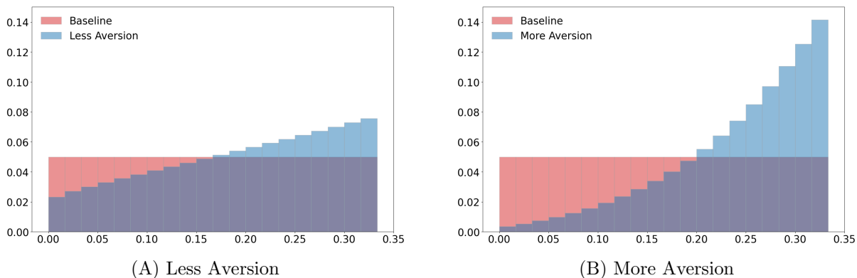
Figure 5: Distorted damage model distribution. The plot shows the undistorted and distorted distributions with less misspecification aversion in the left panel and more misspecification aversion in the right panel. The histograms are calculated at year 0, with the trajectories leading up to year 0 simulated under the baseline dynamics abstracting from the intrinsic randomness.
