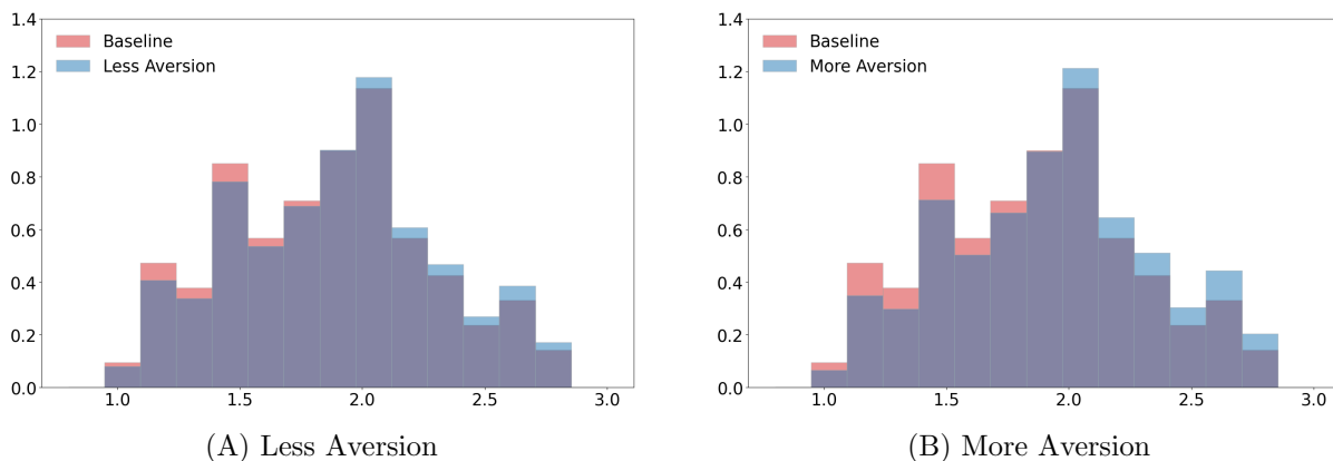
Figure 4: Distorted climate model distribution. The left plot shows the undistorted and distorted distributions with less misspecification aversion. The right plot shows the undistorted and distorted distributions with more misspecification aversion. The histograms are calculated at year 0, with the trajectories leading up to year 0 simulated under the baseline probabilities and abstracting from the intrinsic randomness. Recall that Brownian motion misspecification aversion induces a shift in the local mean. The distorted histograms were constructed by imposing instead ambiguity aversion where the ambiguity penalization was set to capture the same unfavorable conditional mean distortion as the misspecification aversion. See Appendix A.5 for details. The “no aversion” mean of this distribution is 1.86; with less aversion it is 1.88, and with more aversion it is 1.92.
