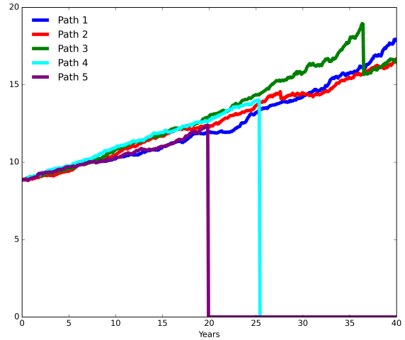
(B) Stochastic Simulation Pathways: E_t
