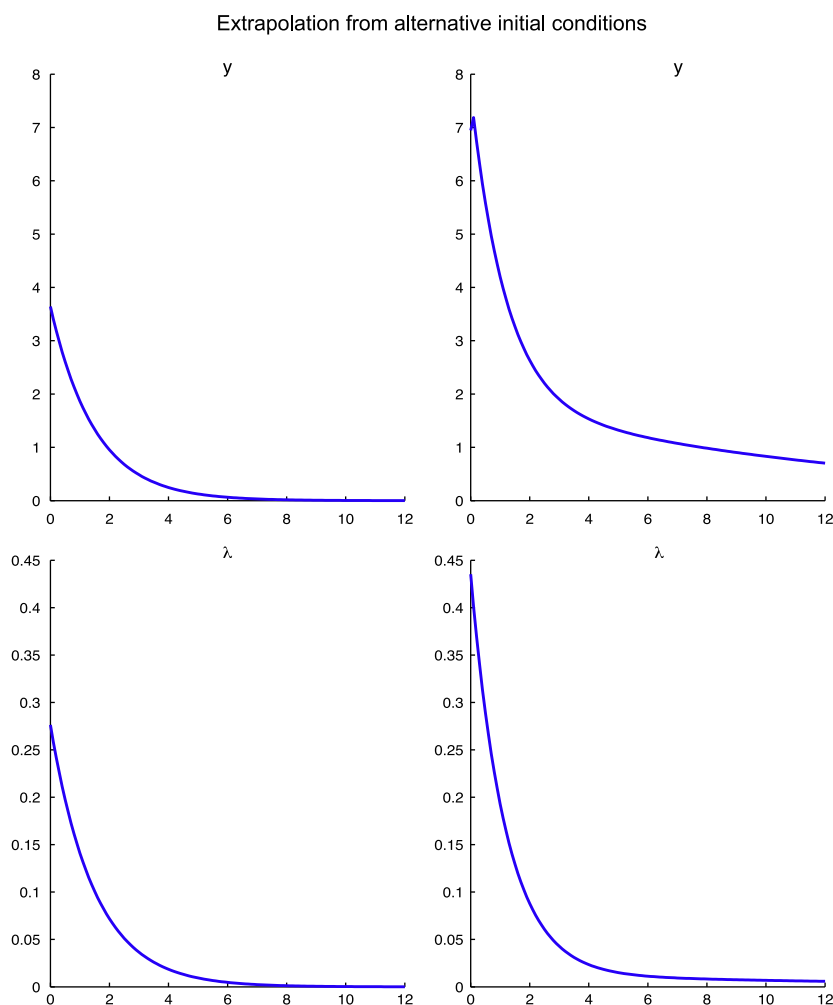
Fig. 3. The left panels assume the approximating model for the cost process initialized at its unconditional mean, 0. The right panels assume the worst-case models for the cost process initialized at its unconditional mean, .0249. The top panels give trajectory differences without shocks for the logarithm of the output gap (times one hundred), and the bottom panels give trajectory differences (times one hundred) for inflation without shocks. The time units on the horizontal axis are quarters.
