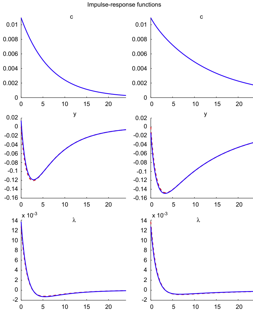
Fig. 2. The left panels assume the approximating model for the cost process, and the right panels assume the worst-case models for the cost process. The top panels give the impulse response functions for the cost process, the middle panels for the logarithm of the output gap, the bottom panels for inflation. The dashed line uses the approximating model solution and the solid line uses the worst-case model solution. The time units on the horizontal axis are quarters.
